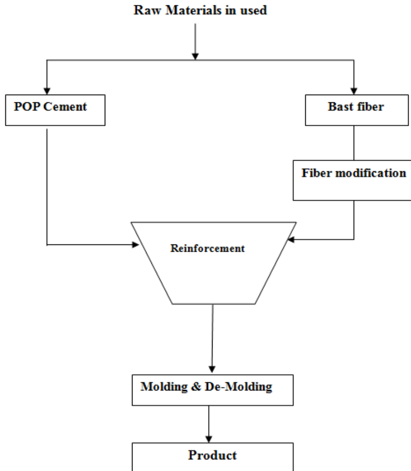
Fig. 1. Process flow diagram
