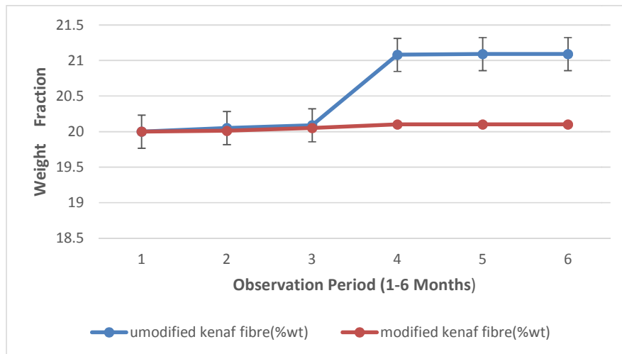
Fig. 8. Effect of moisture movement and environmental stability of reinforced material
