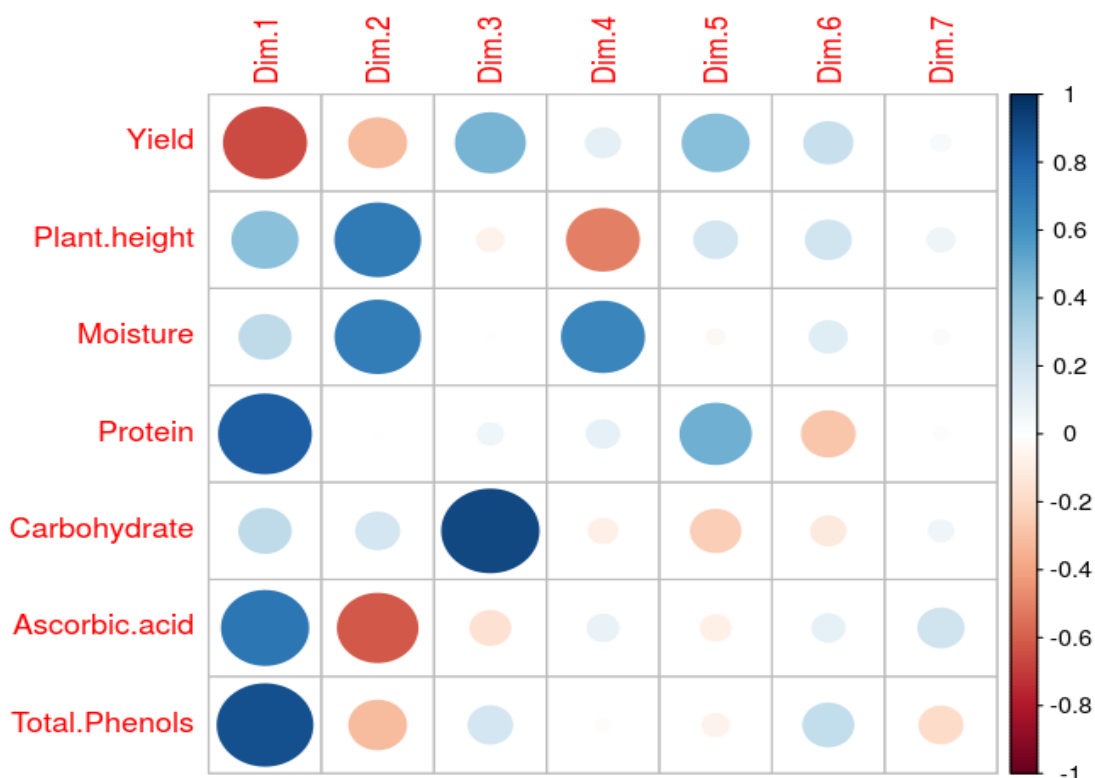
Fig. 1. Correlogram shows the association between the various traits with PCs
