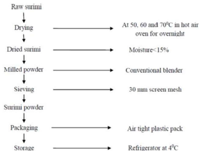
Fig. 2. Flowchart of surimi powder preparation
