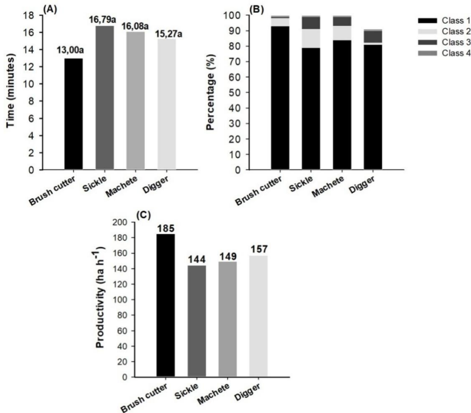
Fig. 2. Average operating time per plot (A), damage percentage in each class (B) and productivity per hectare (C) for each of the evaluated methods
