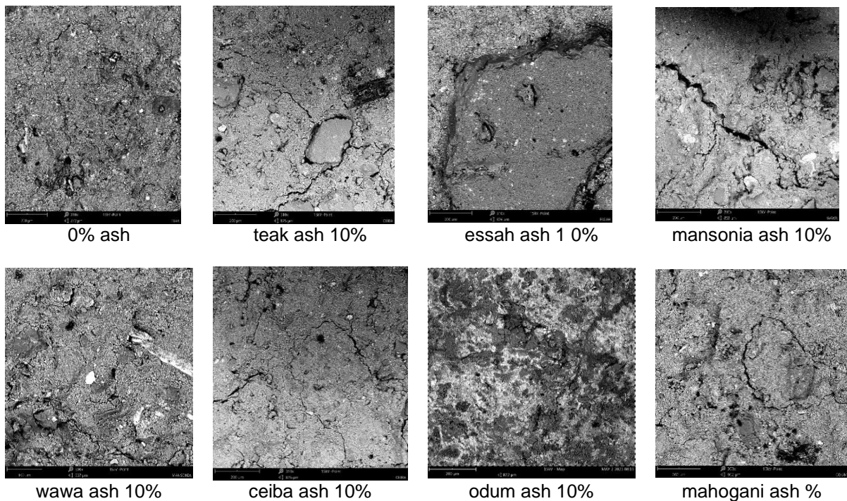
Fig. 10. SEM Images of all the seven BSDA compressed cement-laterite interlocking blocks
