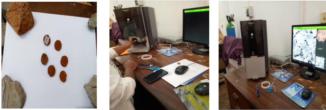
Fig. 5&6. EDS and SEM analysis of compressed laterite interlocking blocks set up
