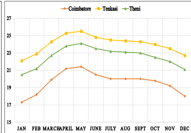
Fig. 5. Mean monthly minimum temperature (°C) over the study regions
