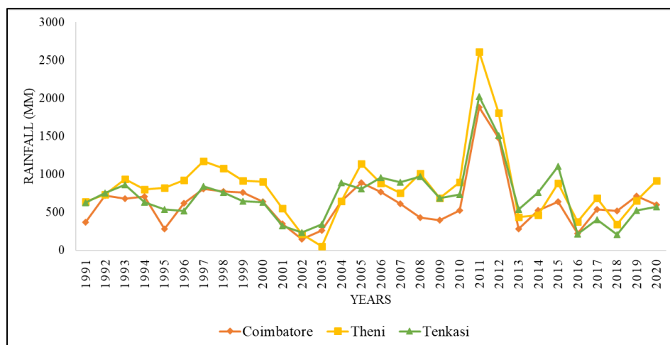
Fig. 3. Annual average rainfall (mm) of regions (1991 – 2020)
